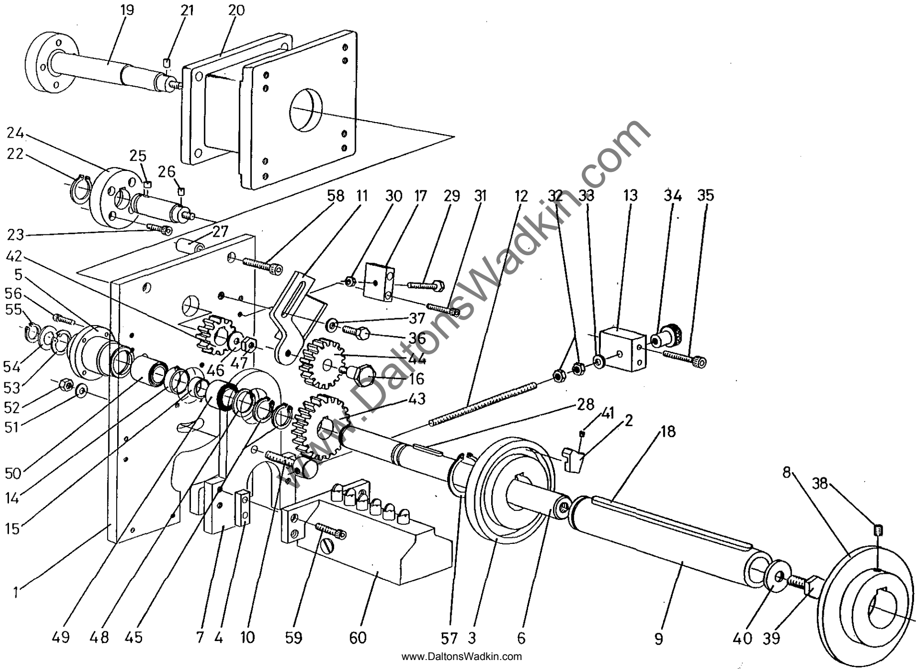
FIG 27 TIMING DRUM
