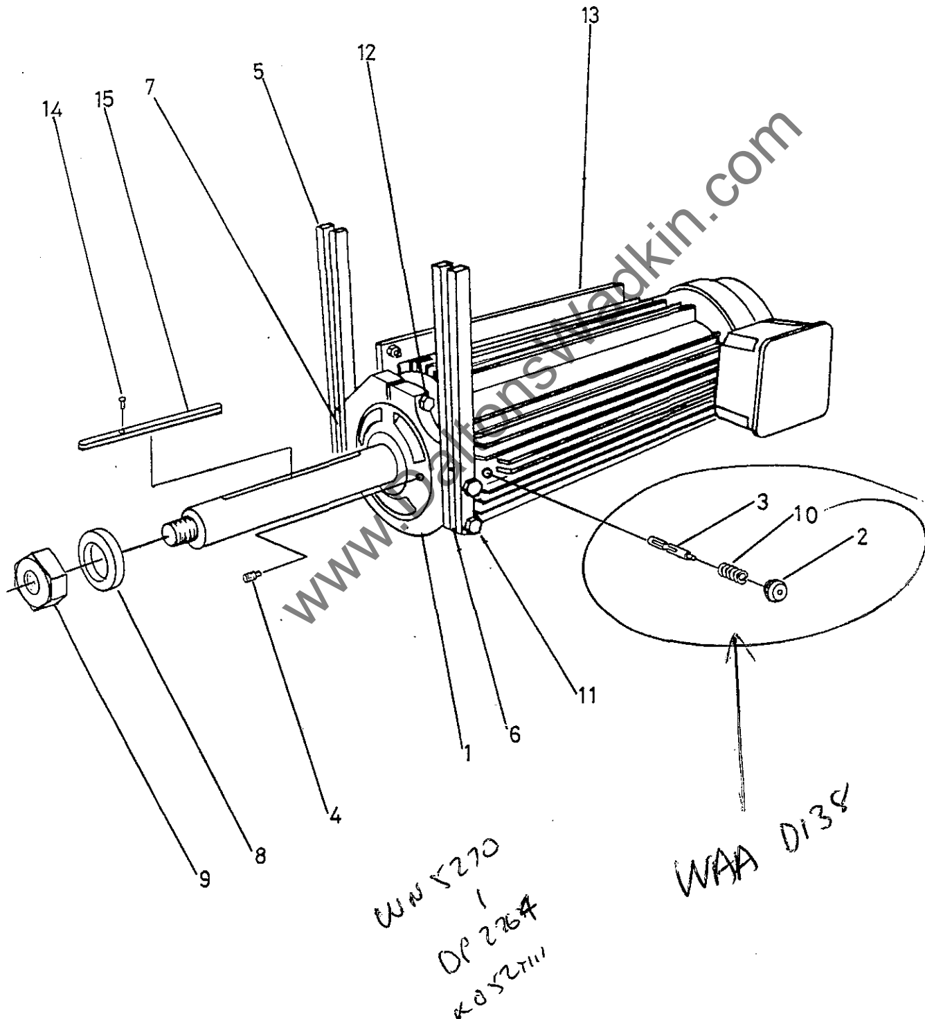
FIG 21 'A' TYPE HEAD
