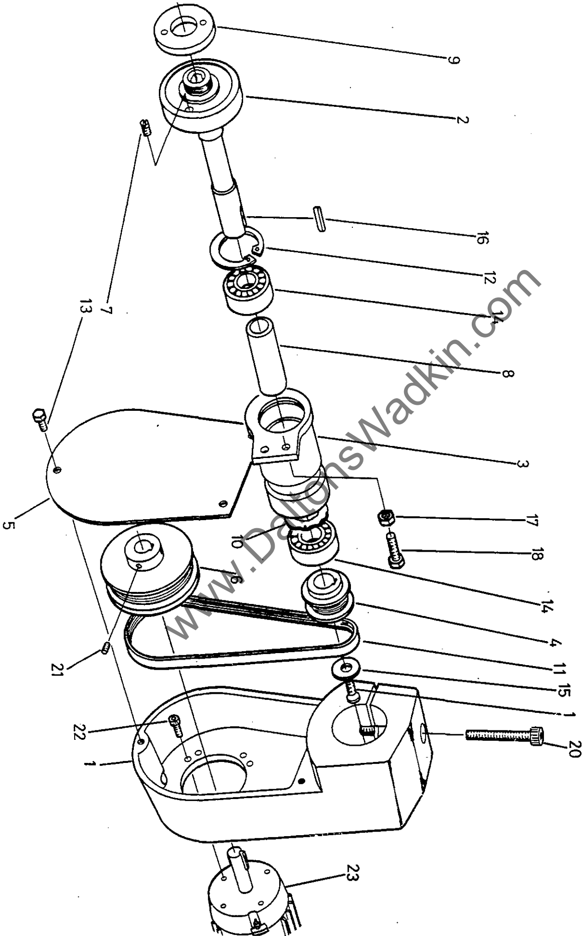
FIG 24 BELT DRIVEN SCORER HEAD
