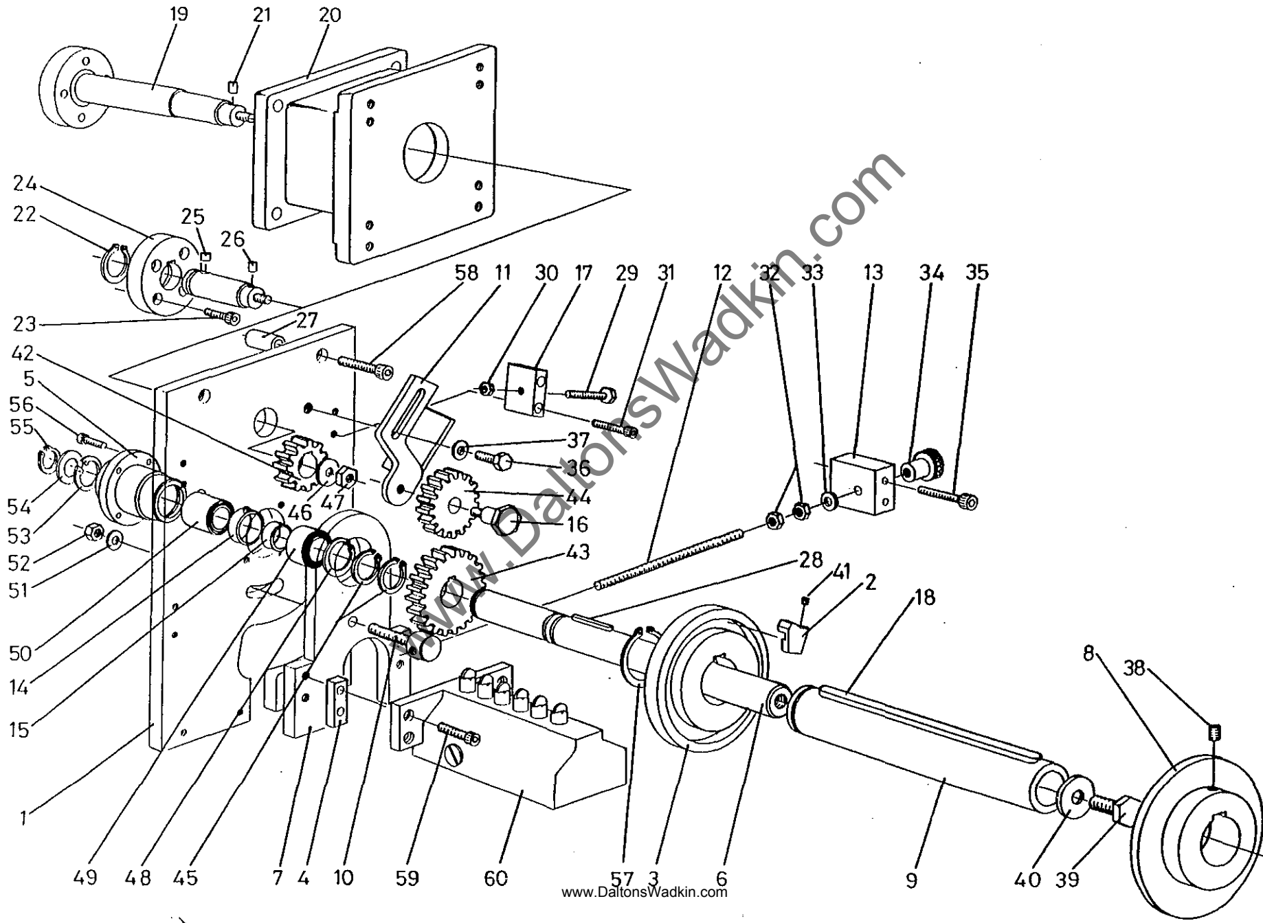
FIG 27 TIMING DRUM
