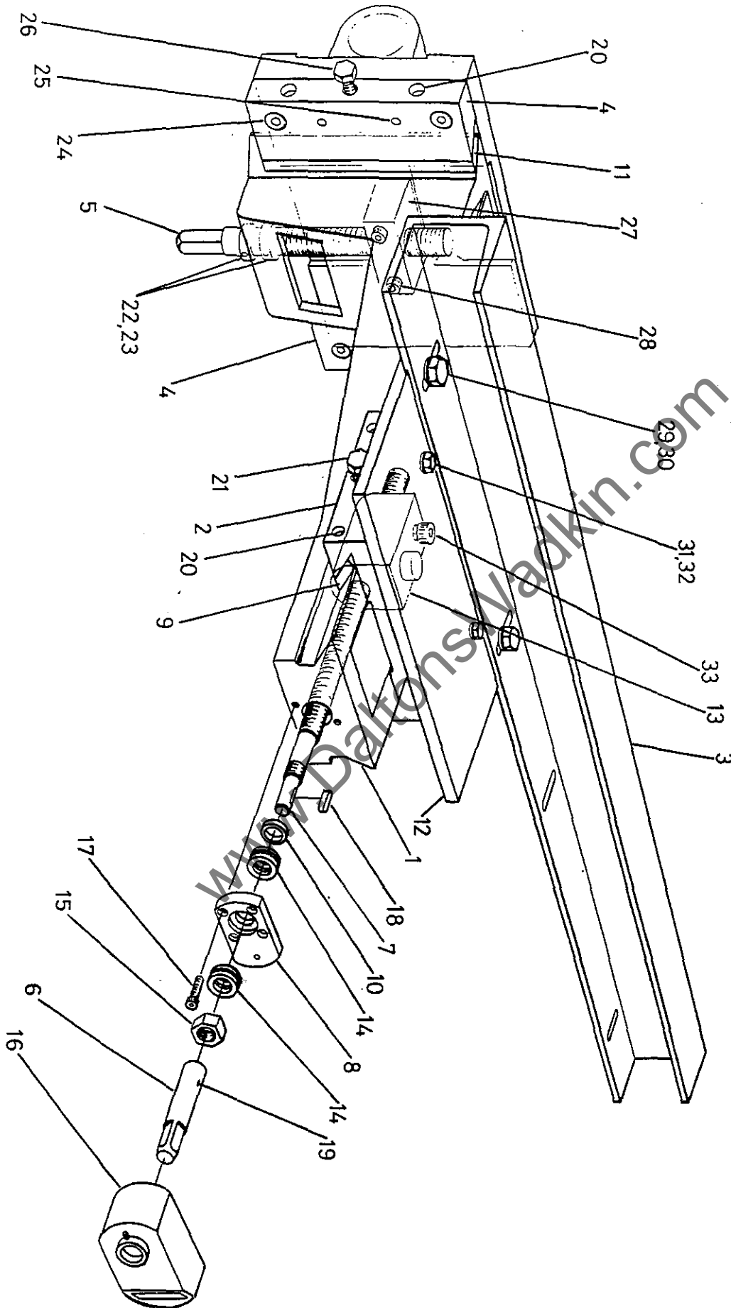
FIG. 20 STANDARD 1.5M INFEED FENCE
