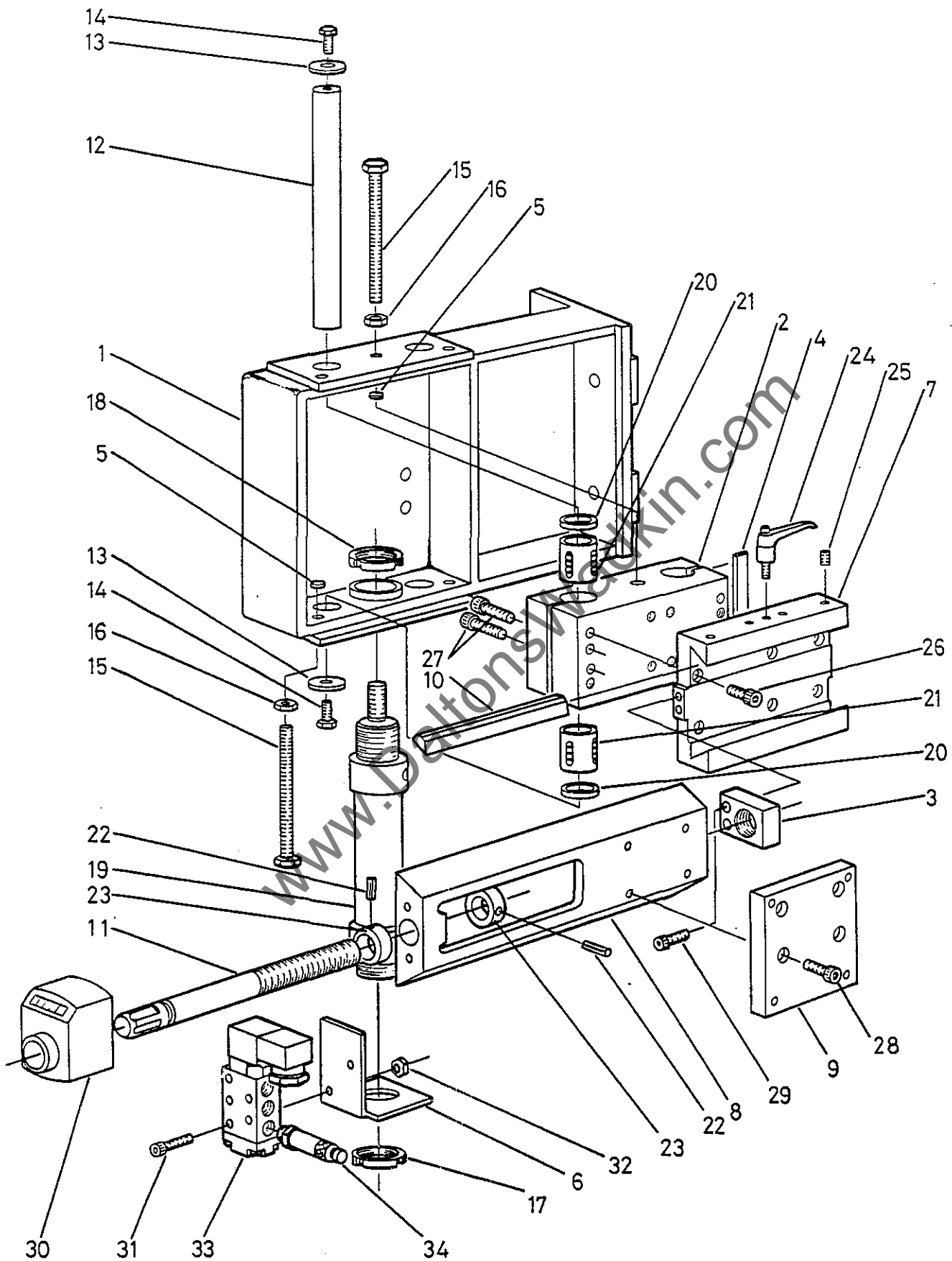
FIG 23 BEAM MOUNTED SCORER BODY
