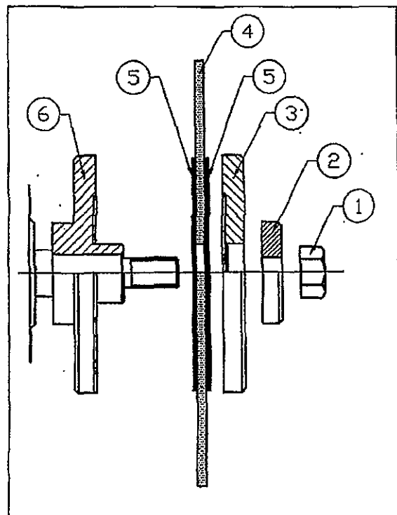
Fig. 4a Grinding wheel mounting
