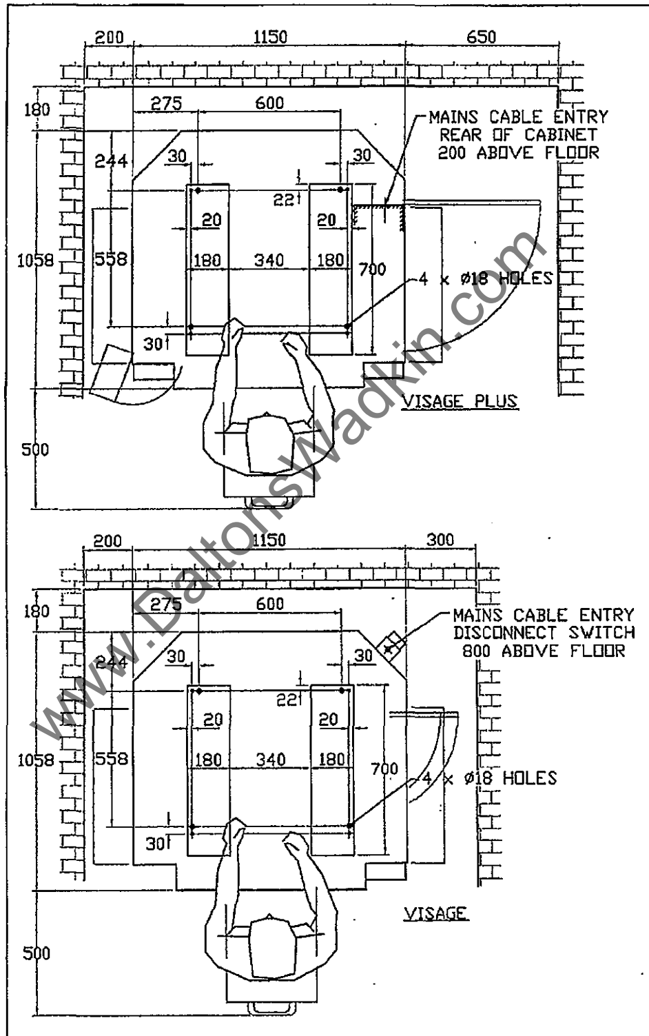
Foundation plan
