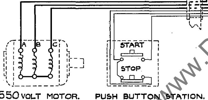
TYPE R.A. SIZE N°1 MAGNETIC STARTER, MOUNTED ON DOOR OF CONTROL GEAR CAVITY.
