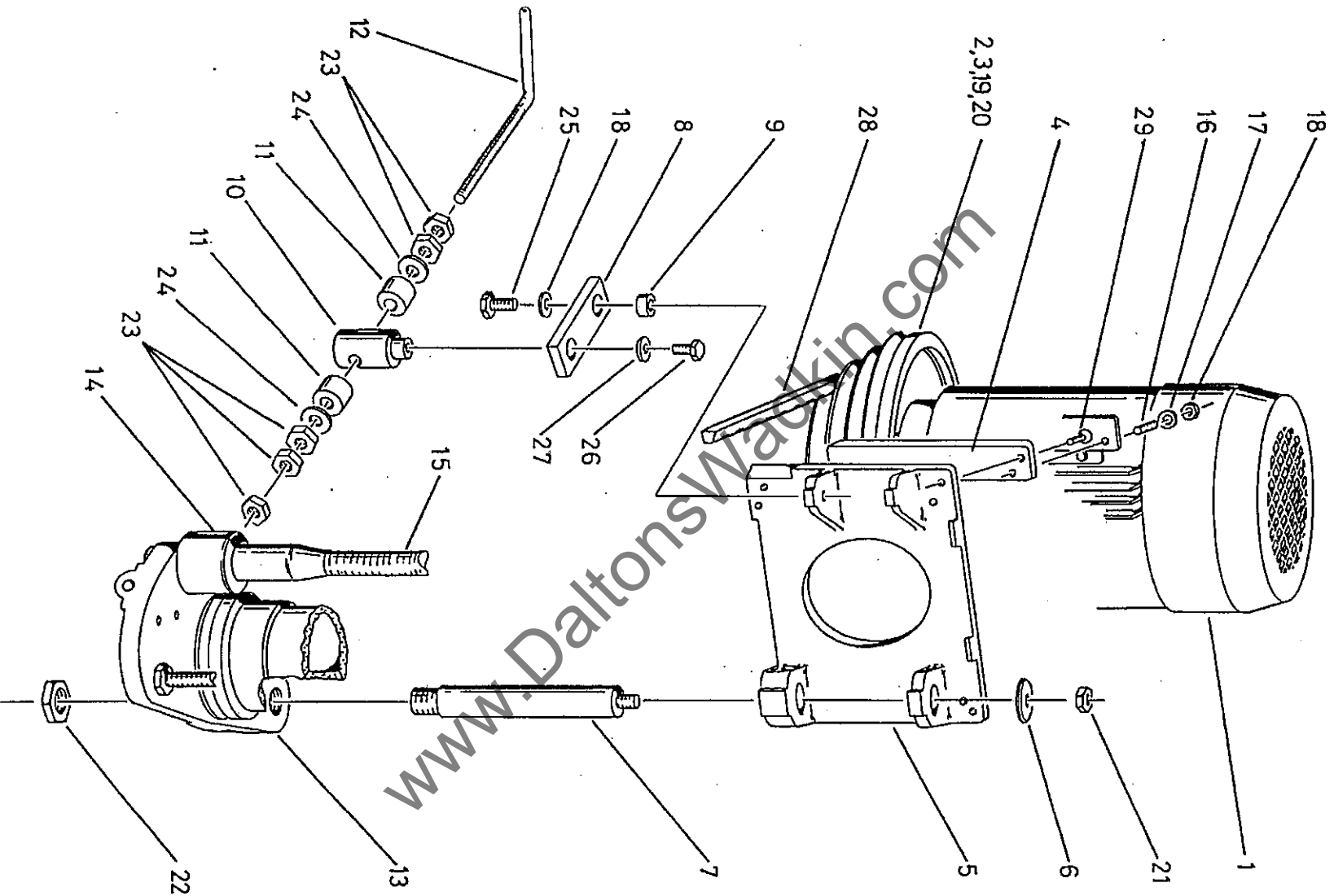
FIG 6 MOTOR MOUNTING AND BELT TENSIONER
