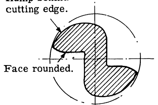
Cutter incorrectly ground and honed.
