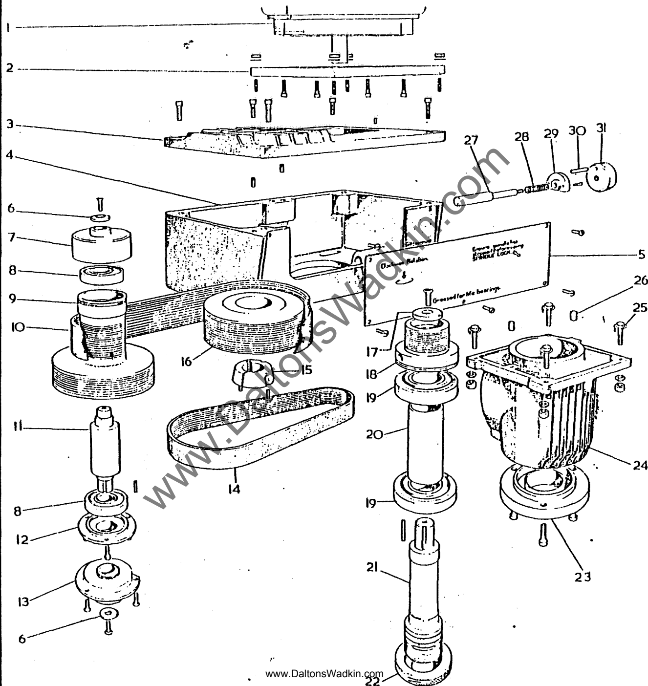
EXPLODED VIEW OF UR/B. ROUTER HEAD
