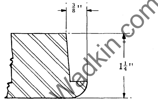
Maximum and minimum sizes of dovetail grooves
