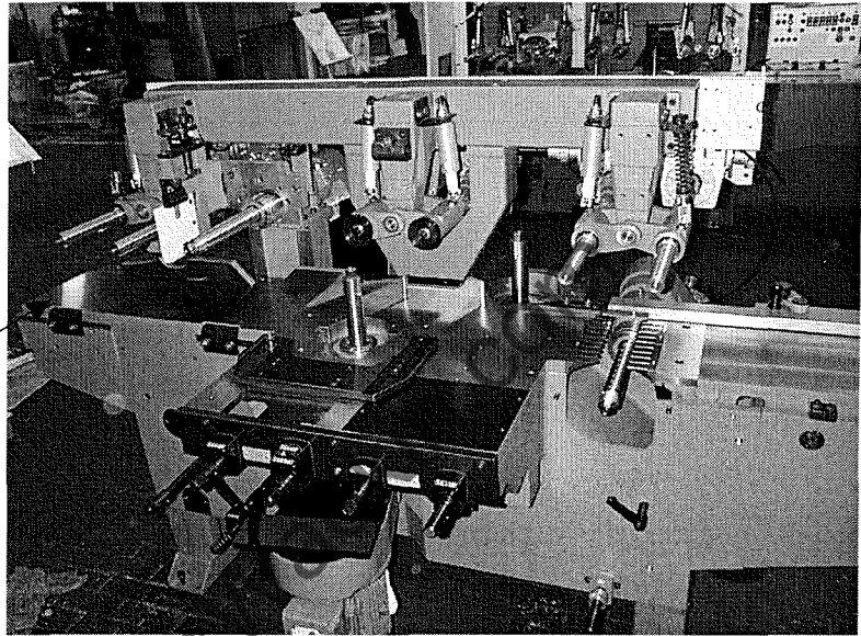
BEDPLATES FOR A FOUR HEAD MACHINE
