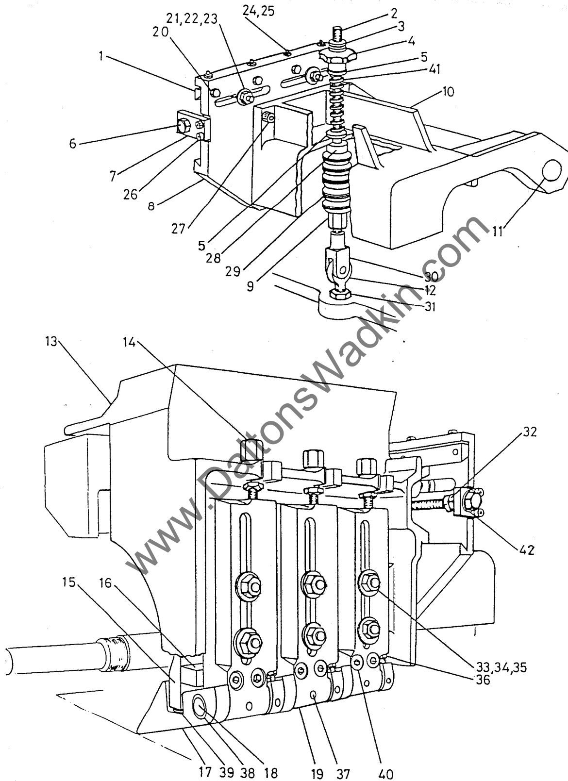
FIG 43 XE E-UNIT (TOP HEAD CHIPBREAKER)
