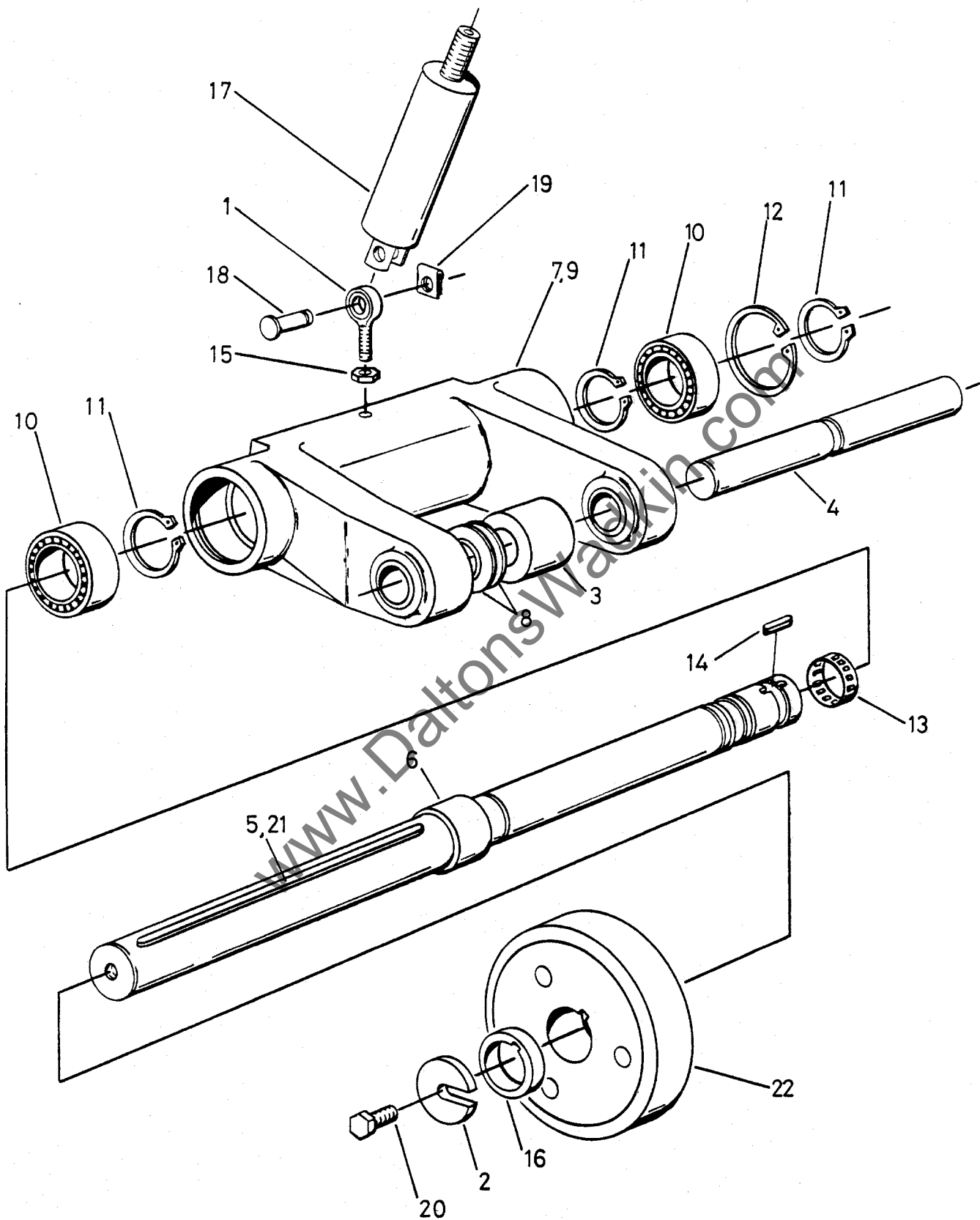
FIG 27 SHAFT MOUNTED FEEDROLL
