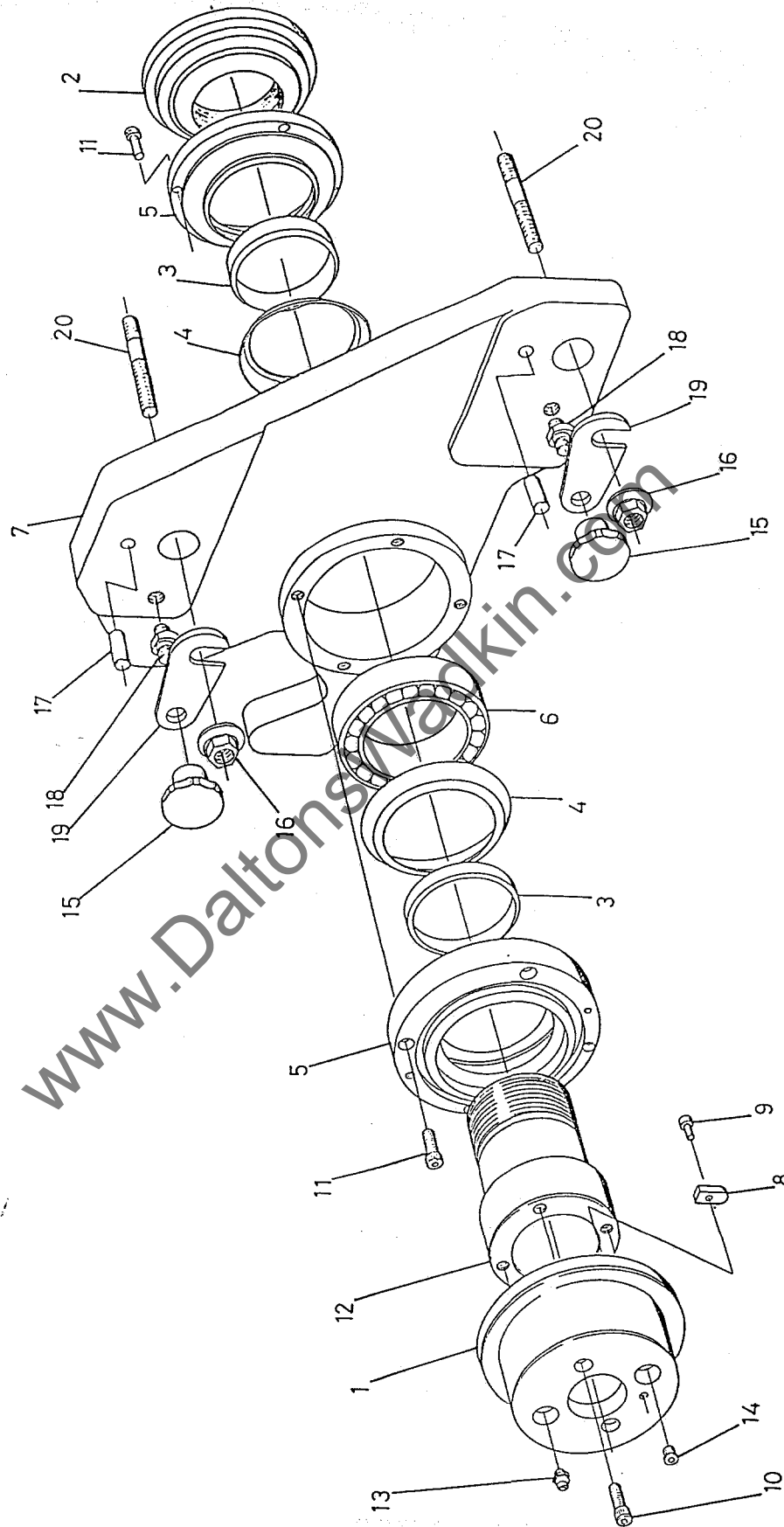
FIG 43 XE E-UNIT (OUTBOARD BEARING TOP HEAD)
