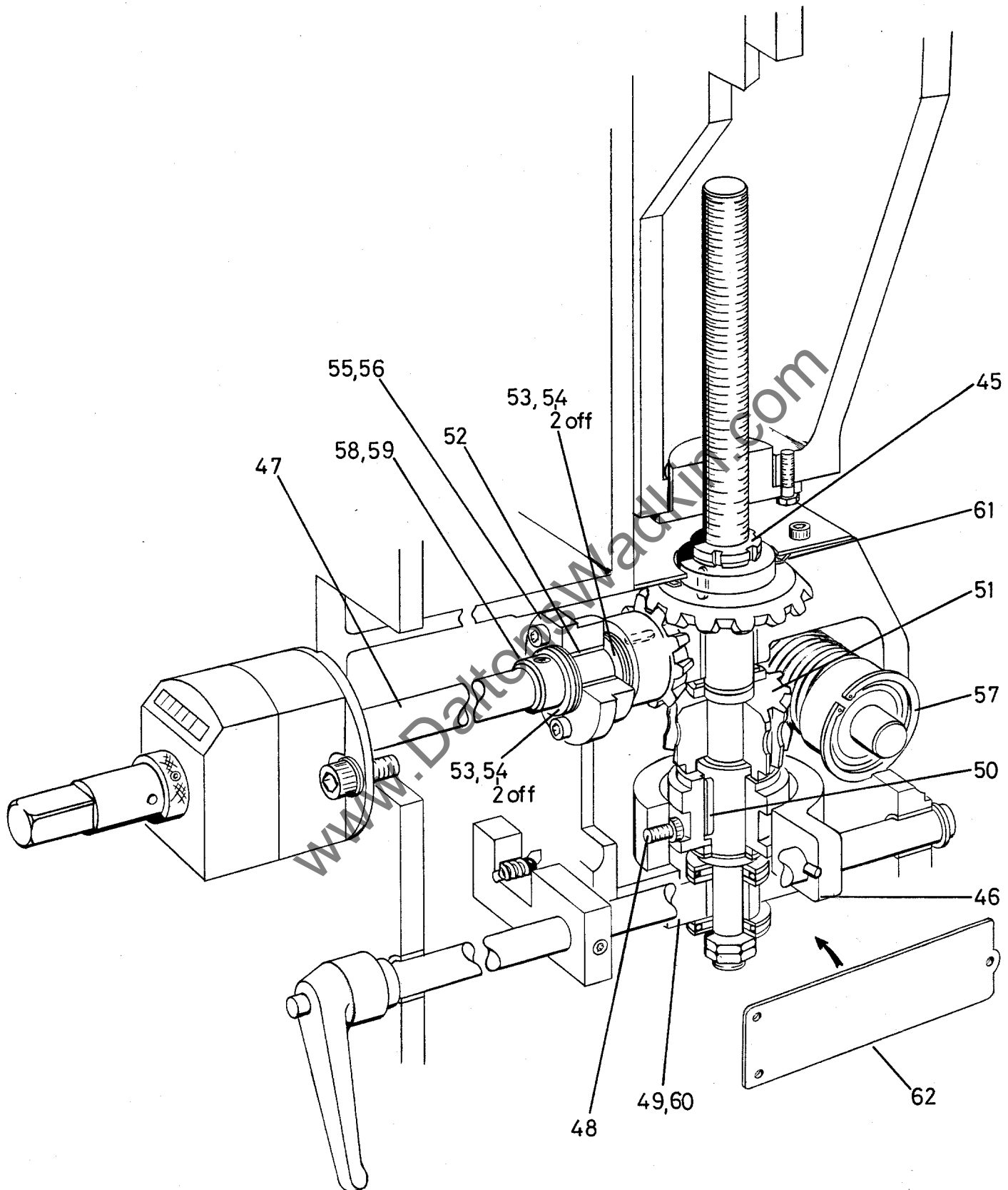
FIG 6 TOP HEAD VERTICAL ADJUSTMENT
