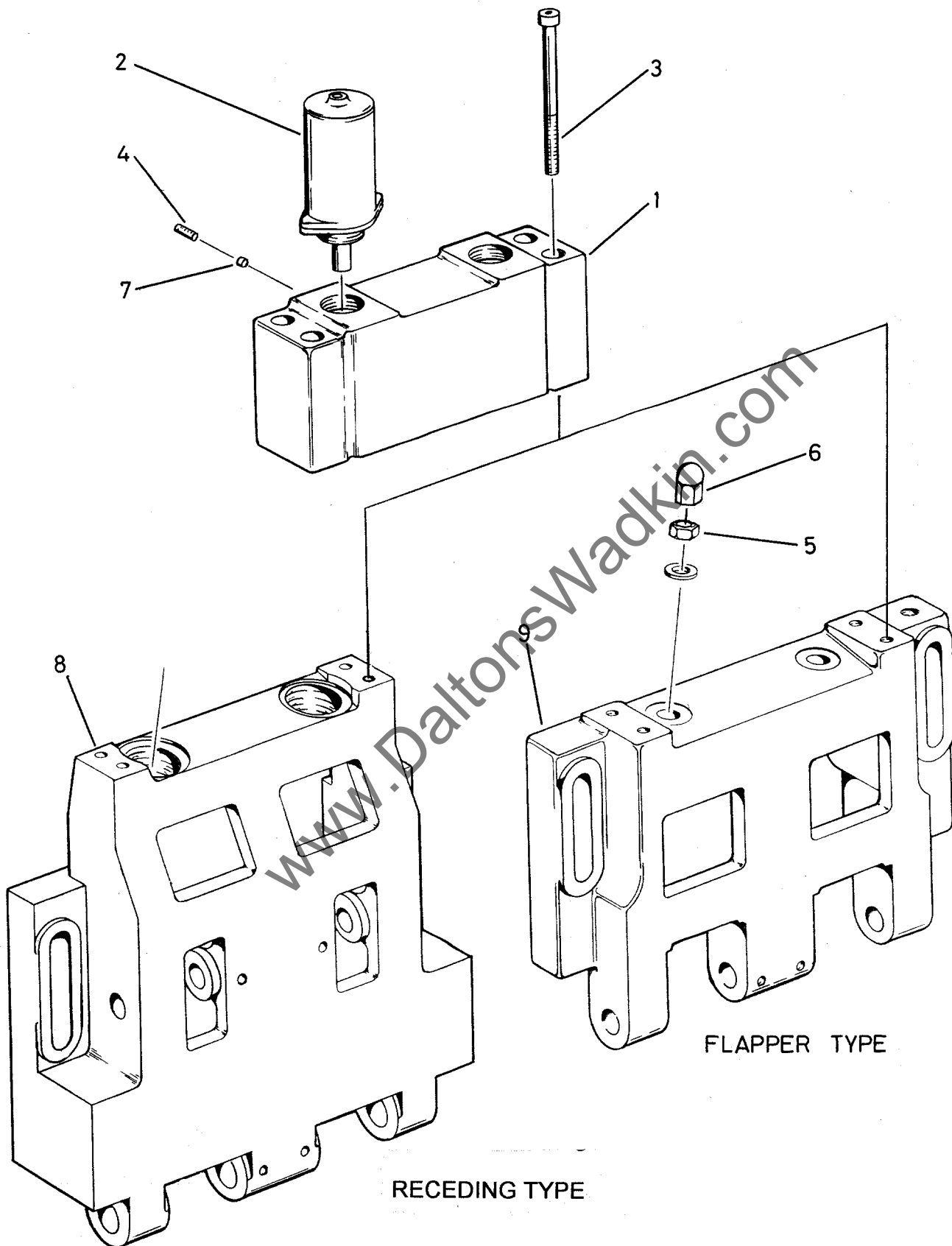
FIG 10 PNEUMATIC CHIPBREAKER — TOP HEAD
