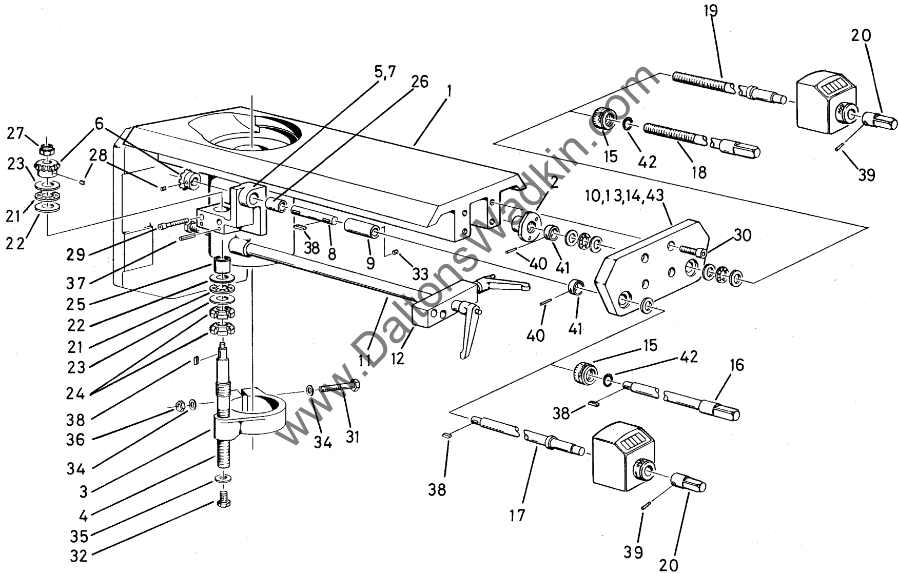
FIG 14 FENCE SIDE AND NEAR SIDE HEAD ADJUSTMENT
