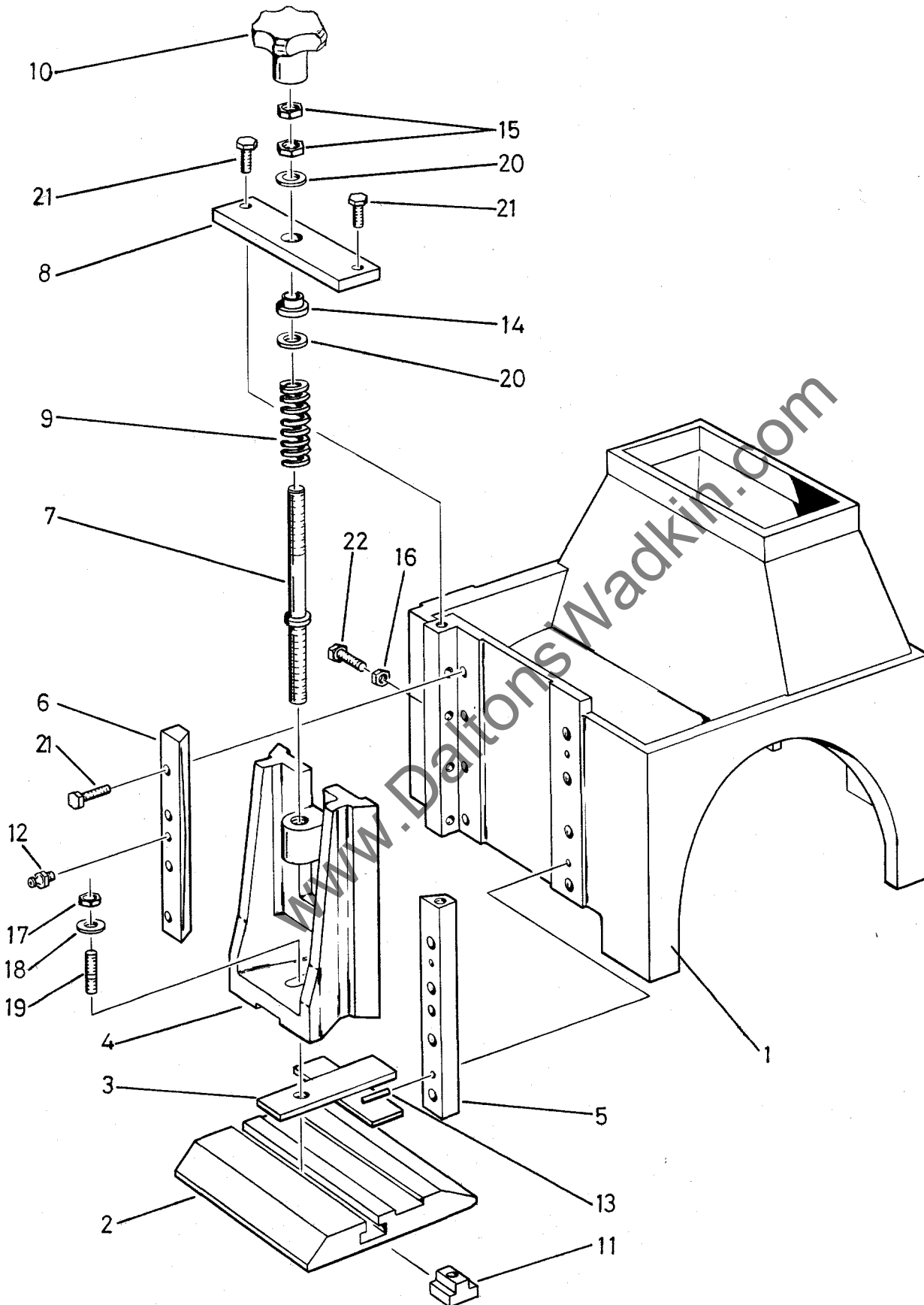
FIG 13 TOP HEAD PAD PRESSURE
