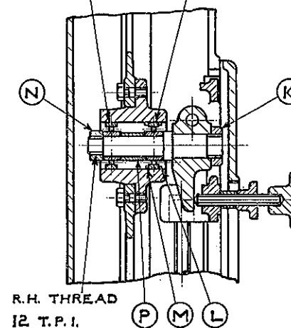
FIG.4 SECTION THROUGH TOP PULLEY SPINDLE.
